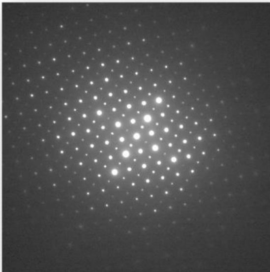
Without precession
