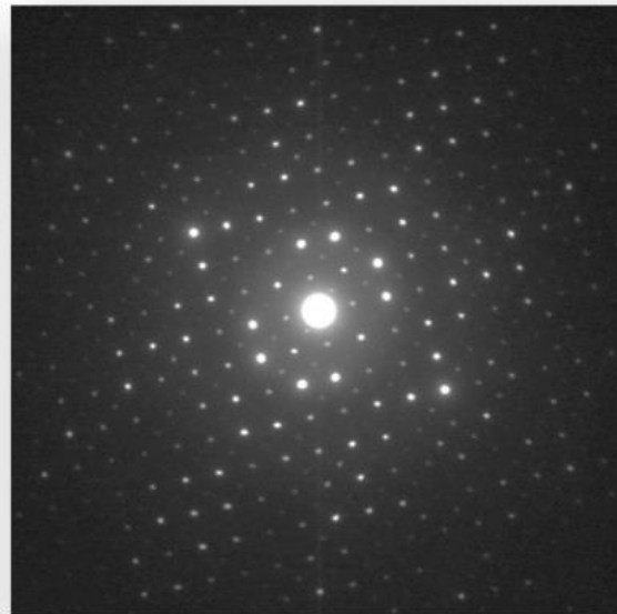
With precession
